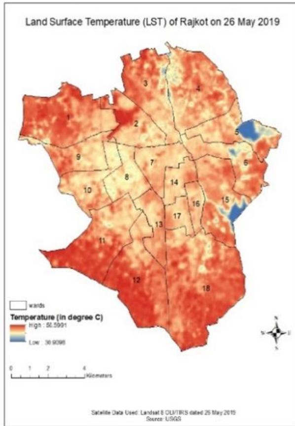
Figure 1: LST maps of three cities developed using satellite data.
