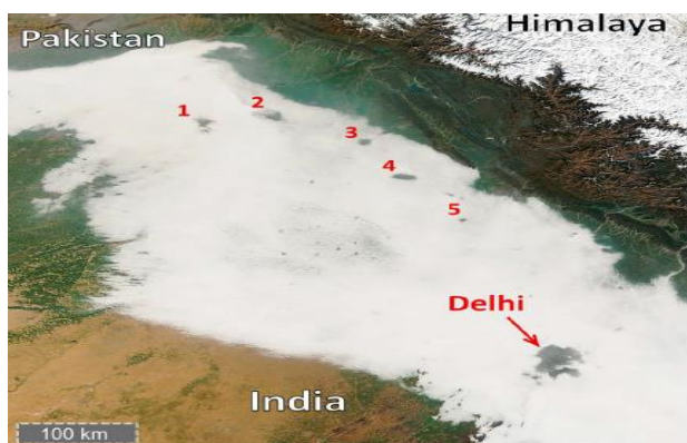
Figure: Satellite image showing fog holes over India and Pakistan with extensive holes over Delhi and several other cities [Lahore (1), Amritsar (2), Jalandhar (3), Ludhiana (4), and Patiala (5)] throughout the IGP, seen from spaceborne MODIS instrument on 30 January 2014 at ~10:30 a.m. local time (Source: Gautam and Singh, 2018).
