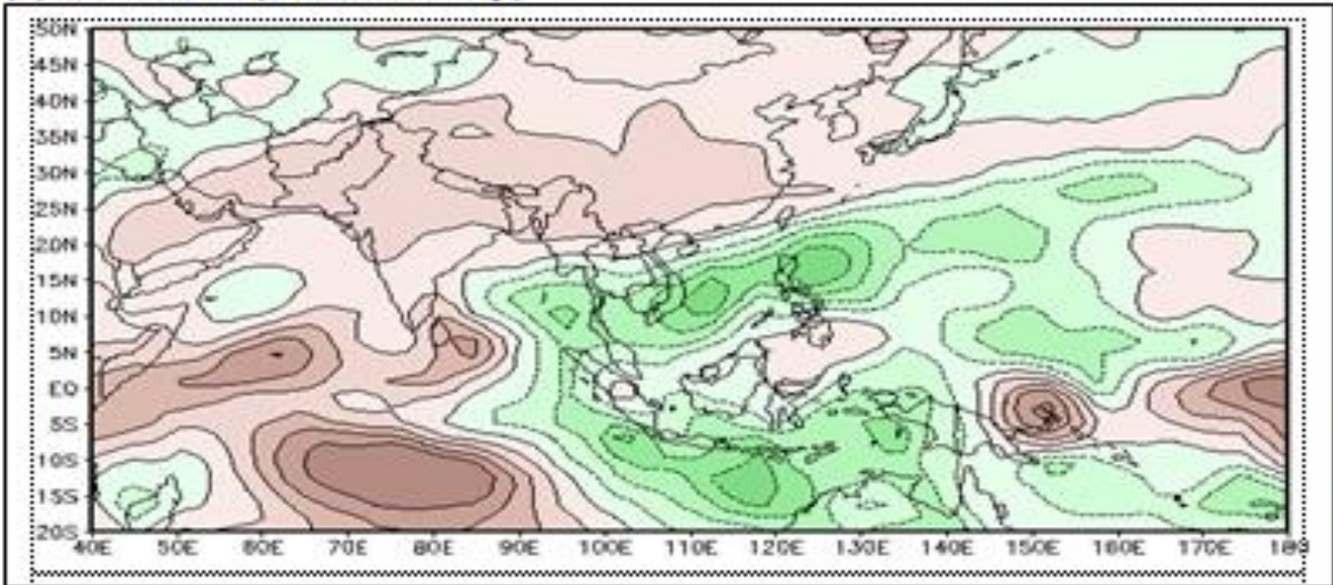
(b) Jan 2017 (OLR anomaly)
