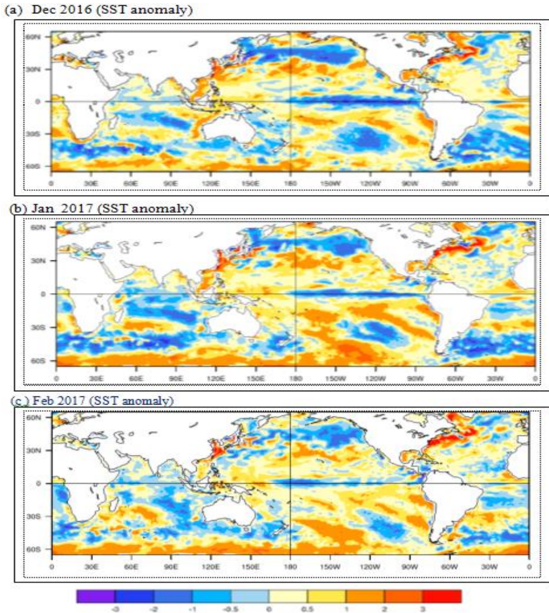
Figure 1: Average SST anomalies (°C) for (a) December 2016, (b) January 2017 and (c) February, 2017. (Data source: INCOIS-GODAS).
