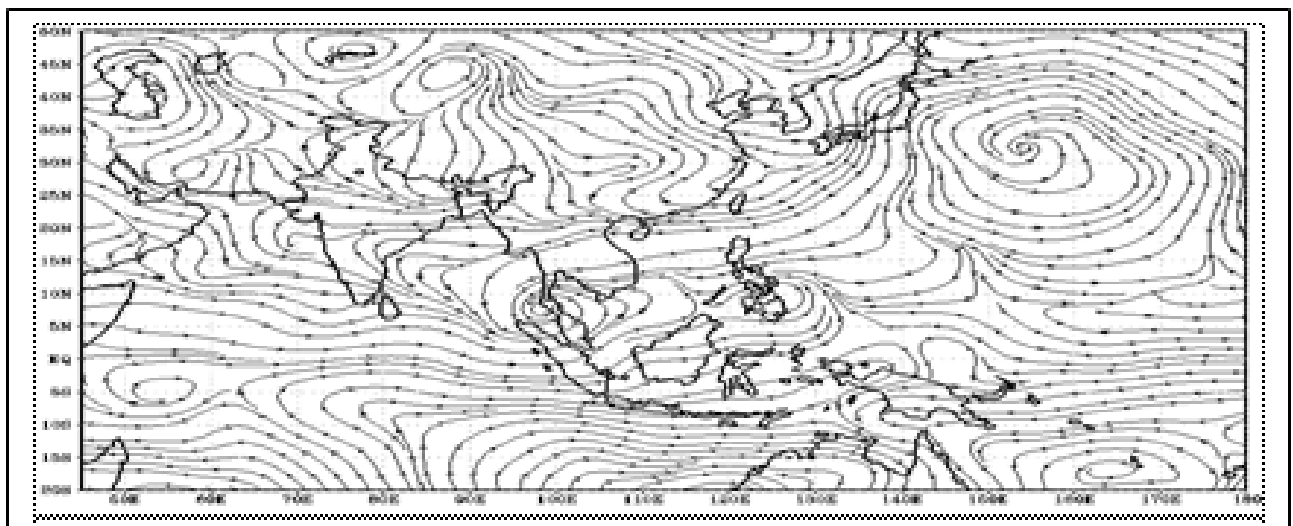
(c) Feb 2017 (850 hPa wind anomaly)
