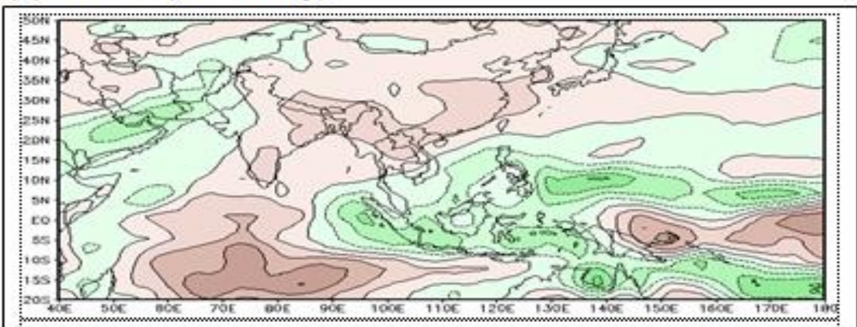
(c) Feb 2017 (OL anomaly)
