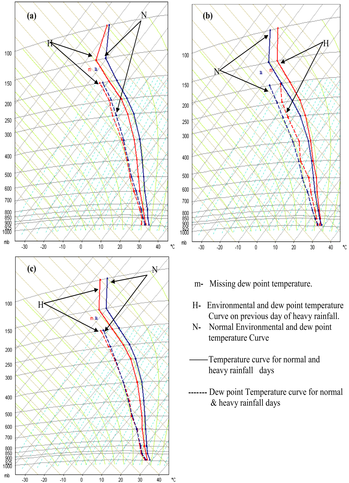
Figure 3: Thermodynamic Characteristics over (a) Gorakhpur (b) Lucknow & (c) Patna associated with heavy rainfall over East-UP.
